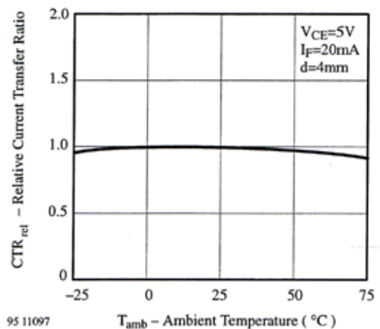
Figure 4. Rel. Current Transfer Ratio vs. Ambient Temperature
