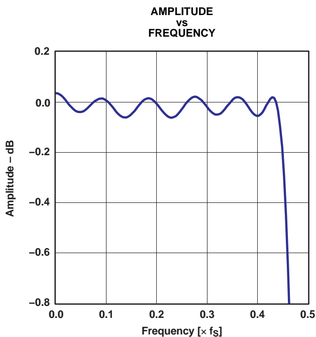
Figure 25. Pass-Band Ripple
